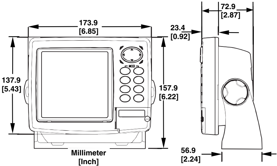
Front view (left) and side view (right) showing dimensions of the GlobalMap 3500C when mounted on gimbal bracket.
