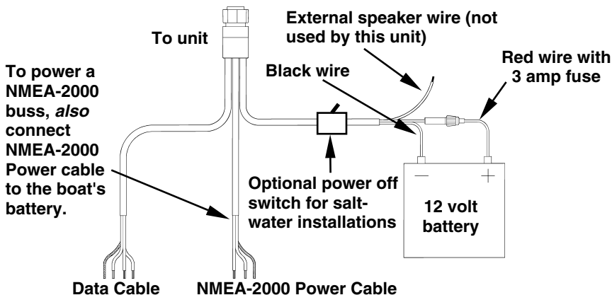
Power connections for the GlobalMap 3500C GPS unit.
