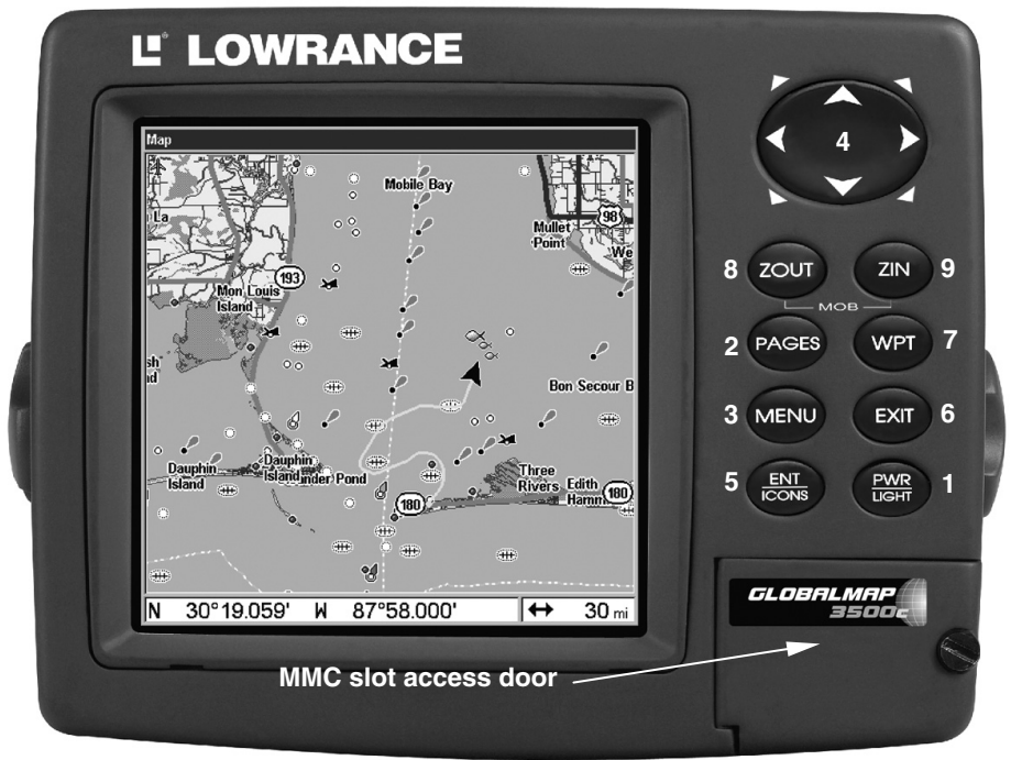
GlobalMap 3500C GPS unit, front view, showing Map Page, keyboard and access door for the MMC slot.
